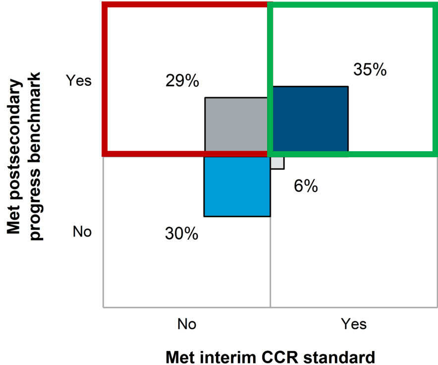
Classification rates: Predicting PSY1F credits \geq 12
