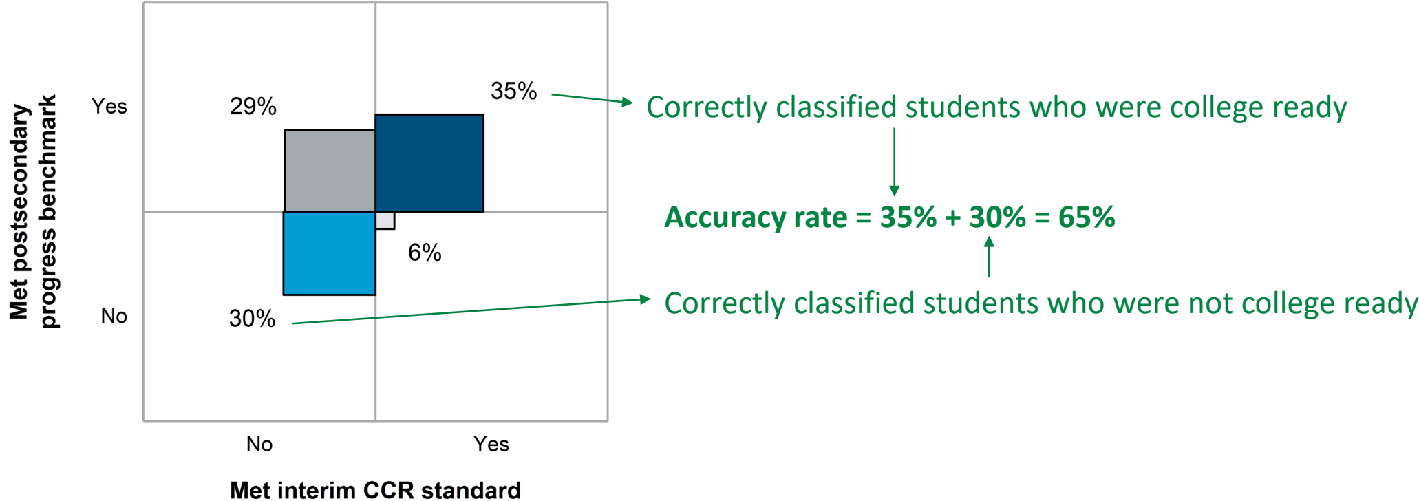
Classification rates: Predicting PSY1F credits \geq 12
