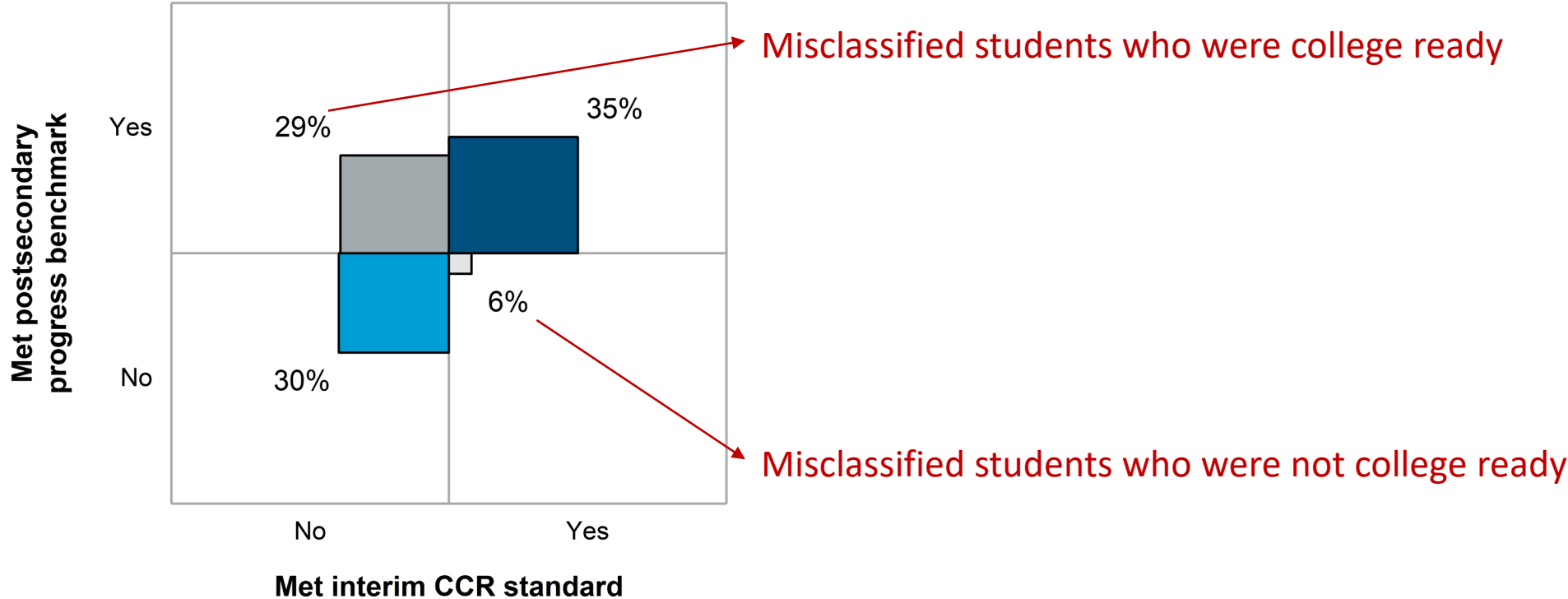
Classification rates: Predicting PSY1F credits \geq 12
